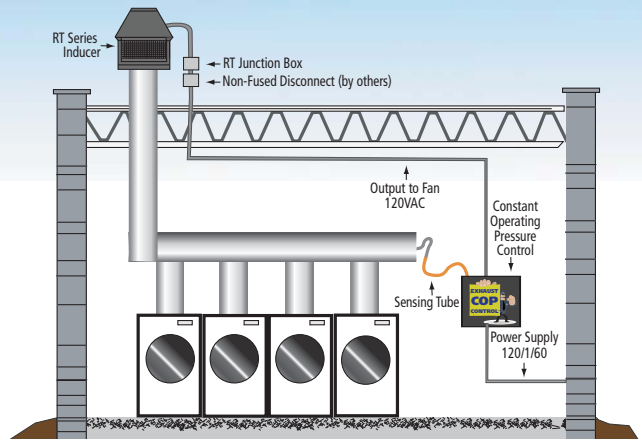
Mutiple Clothes Dryers Common Vented
